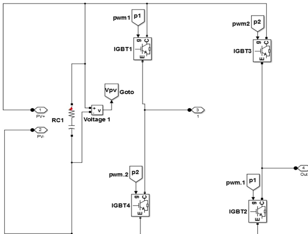
(b) inverter
