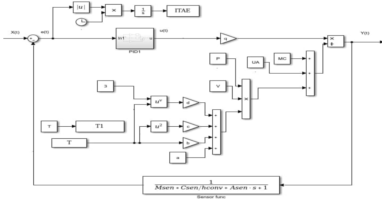
Fig. 4. control on indoor temperature of selected building by using PID with GA (ITAE objective function).
