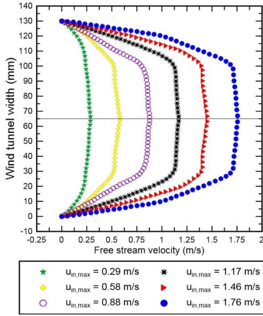
Figure 2. Free stream velocity profile in low-speed wind-tunnel.
