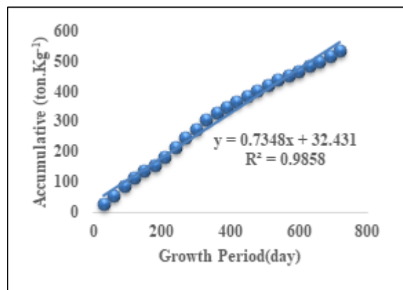
Figure 6. effect of period growth on accumulation of potassium uptake.
