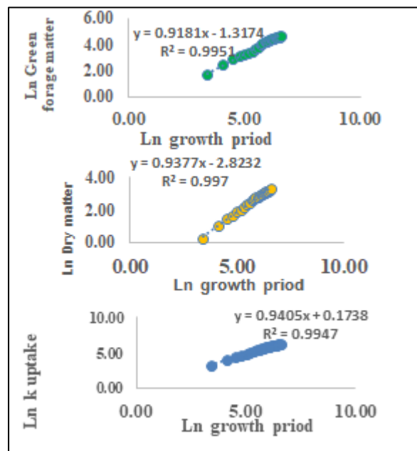
Figure 7. Statistical relationship between green , dry matter and K uptake and crop growth period according to the power function equation.
